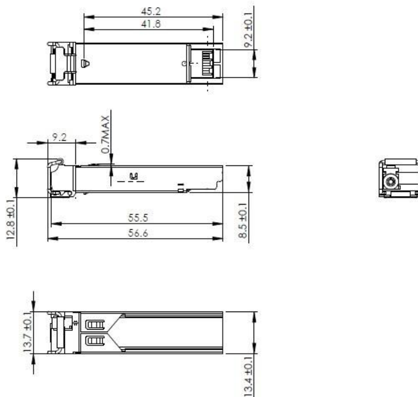
Mechanical Drawing
